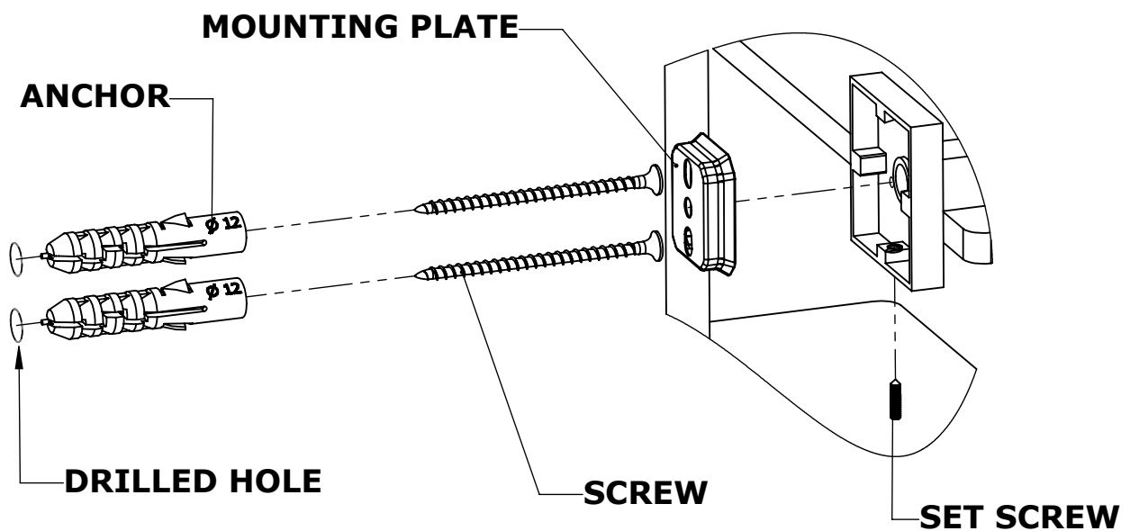
DETAIL M
